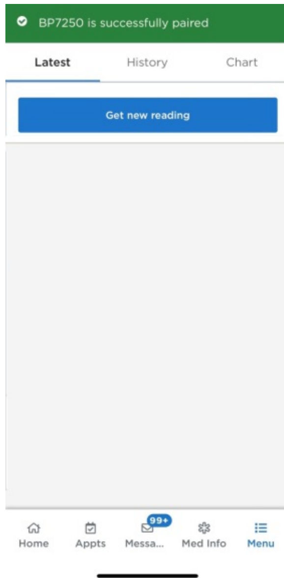
Figure 9. Successful connection
